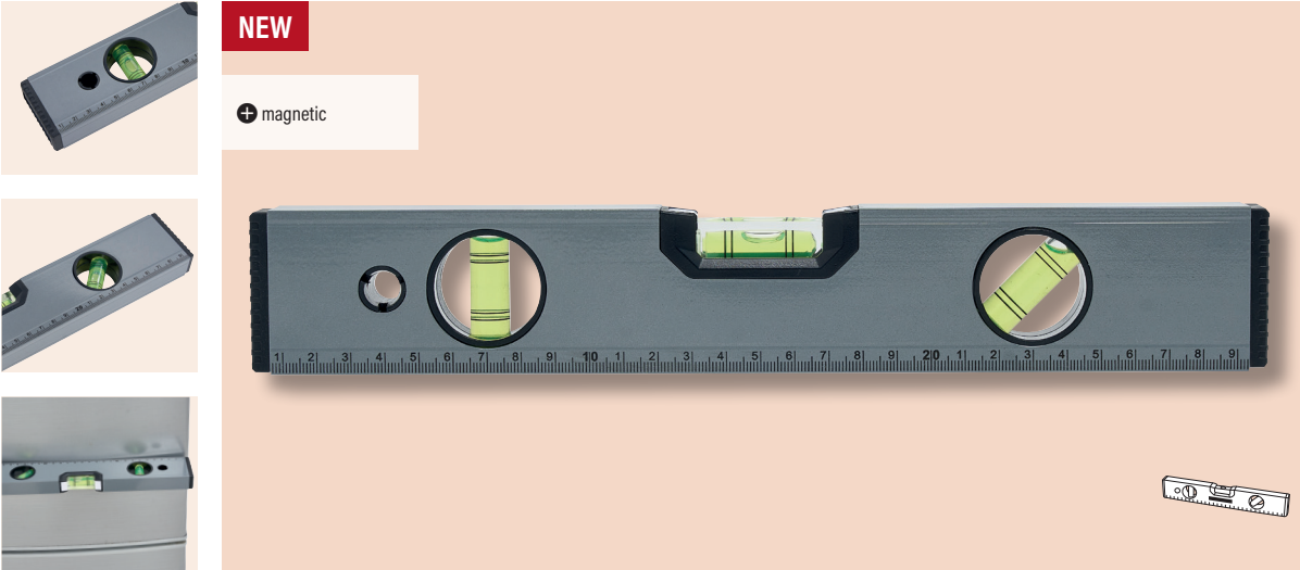
56-0380008 SODALITE Spirit level Packing: 20/40 pcs. | Size: 30x5x2 cm | Material: Aluminium / Acrylic / Plastic | Branding: 5 cm 2 LY5+H2 (1) Spirit level: made of aluminium, 3 separate vials for horizontal, vertical, and 45 ° alignment, printed scale of 30 cm, integrated magnet for easy attachment to metal surfaces, with rubber end caps, in a box
